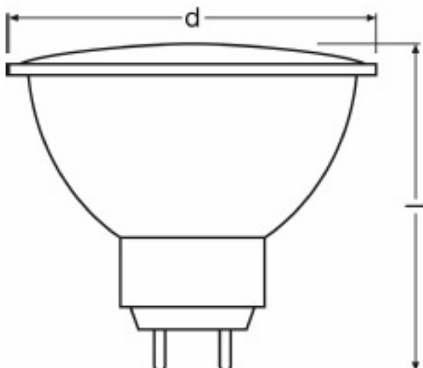
Product line drawing with letters 50 W 12 V 36° GU5.3
